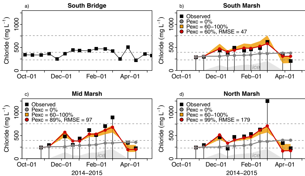
Fig. 3. (a) Chloride concentrations at South Bridge inlet. (b-d) Chloride concentrations at South-, Mid-, and North Marsh from late Oct 2014 to May 2015. Droplines are provided to show sampling dates. Black squares denote observed values while gray circles/line represent modeled chloride concentrations given 0% ion exclusion ( P_{exc} = 0\% ) during ice thickening. The yellow area represents the range in modeled chloride concentrations given rejection rates between 60% and 100%. Red circles/lines represent the best model fit (lowest RMSE). Dashed horizontal lines denote the WI DNR’s acute ( 757 \text{ mg L}^{-1} ) and chronic ( 395 \text{ mg L}^{-1} ) chloride water quality criterion, and the EPA’s chronic water criteria ( 230 \text{ mg L}^{-1} ). Ice thickness is represented by a gray polygon (not to scale).
