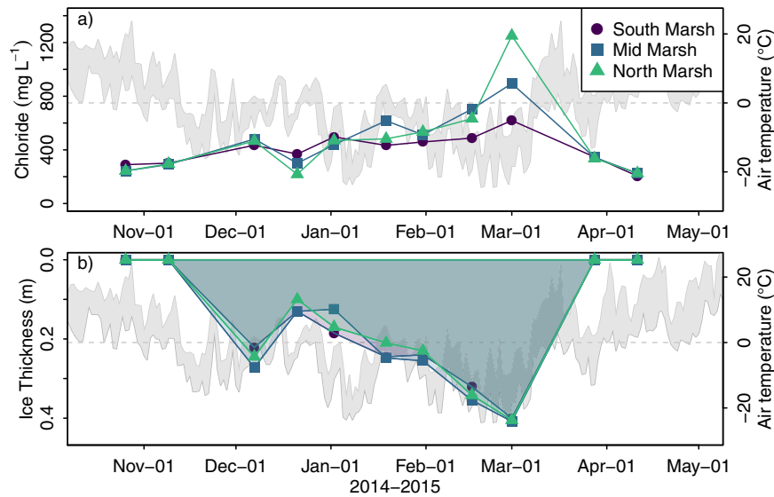
Fig. 2. (a) Chloride concentrations in South-(circles), Mid-(squares), and North Marsh (triangles) from Oct 2014 to May 2015. The gray timeseries represents the range in daily air temperature. (b) Symbols denote the measured ice thickness at the three sites. The lines and shaded area represent the seasonal ice thickness.
