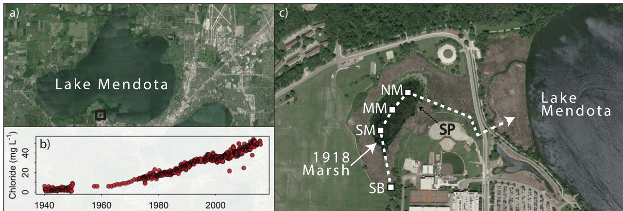
Fig. 1. (a) Lake Mendota (39.6 km 2 ) borders the city of Madison, Wisconsin, U.S.A. Outlined by the black box is the 1918 Marsh, a small marsh (0.074 km 2 ) on the south side of Lake Mendota. (b) Red circles represent chloride concentrations in Lake Mendota. Chloride has been increasing steadily since measurements began in the 1940s. (c) Water flows through the 1918 Marsh from South to North and into Lake Mendota. Sampling sites included South Bridge (SB), South Marsh (SM), Mid Marsh (MM), and North Marsh (NM). The campus snow storage pile (SP) is located immediately east of the marsh. Water drains from the snow pile toward North Marsh.
