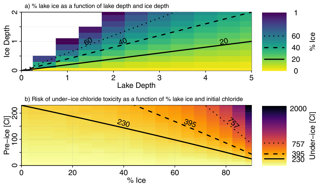
Fig. 4. Risk assessment for chloride toxicity in waterbodies. (a) The amount of lake ice as a percentage of total depth (% ice) is determined based on ice depth vs. lake depth. The solid, dashed, and dotted lines represent the graphical area with 20%, 40%, and 60% ice. (b) Comparing % ice with pre-ice (or summer time) chloride concentrations can determine the risk of under-ice chloride toxicity. Any depth and concentrations units may be used to interpret this figure. Exclusion rate was set at 90%. If concentrations are measured in \text{mg L}^{-1} , lakes that fall to the right of the solid 230 \text{mg L}^{-1} line represent increasing risk from no effect with continuous exposure to noticeable effects of exposure. For example, if lake ice is more than 40% of the lake depth, under-ice chloride concentrations would reach toxic levels ( > 230 \text{ mg L}^{-1} ) if pre-ice concentrations were greater than 140 \text{ mg L}^{-1} . As the percent of ice increases, the pre-ice chloride concentration that would develop toxic winter levels, decreases.
